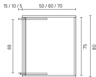
base portalavatrice washing machine base
