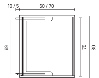
colonna portalavatrice e ripiani tall unit for washer and shelves
