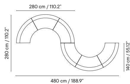
6 curved modules
