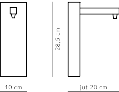
RECTANGULAR WOODEN BRACKET
