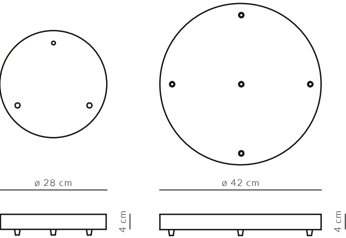
ROUND WOODEN CEILING LIGHTS MOUNT
