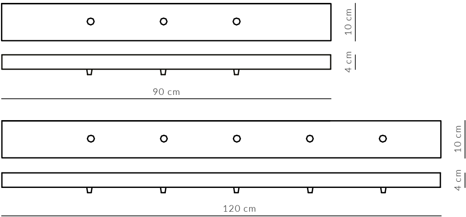
RECTANGULAR WOODEN CEILING LIGHTS MOUNT
